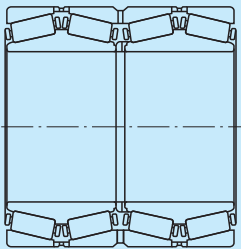
With Pin Type Cages Figure 2
