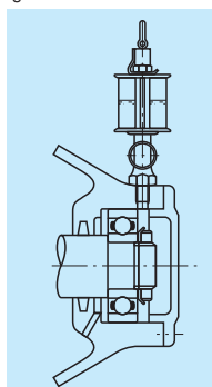
Fig. 4.4 Drip Feed Lubrication
