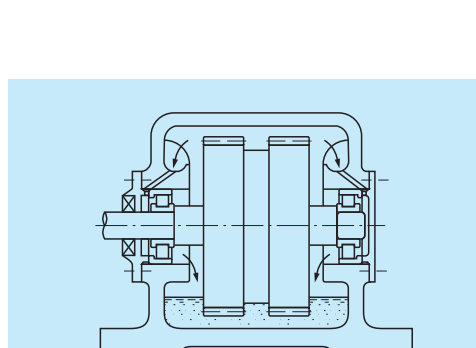
Fig. 4.5 Splash Lubrication
