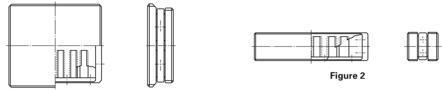
Structure of Converter Trunnion Necks
