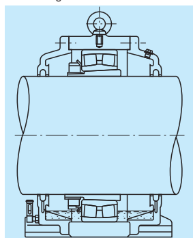
Fig. 4.3 Oil Bath Lubrication
