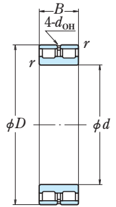
Free-End Bearing RSF
