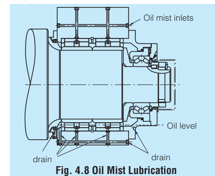
Fig. 4.8 Oil Mist Lubrication
